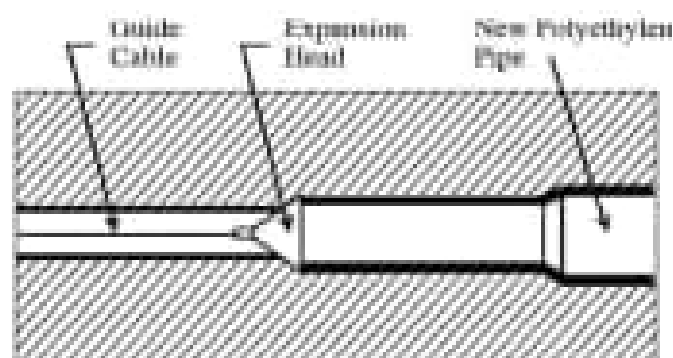
Figure 2.33 Pipe bursting process
