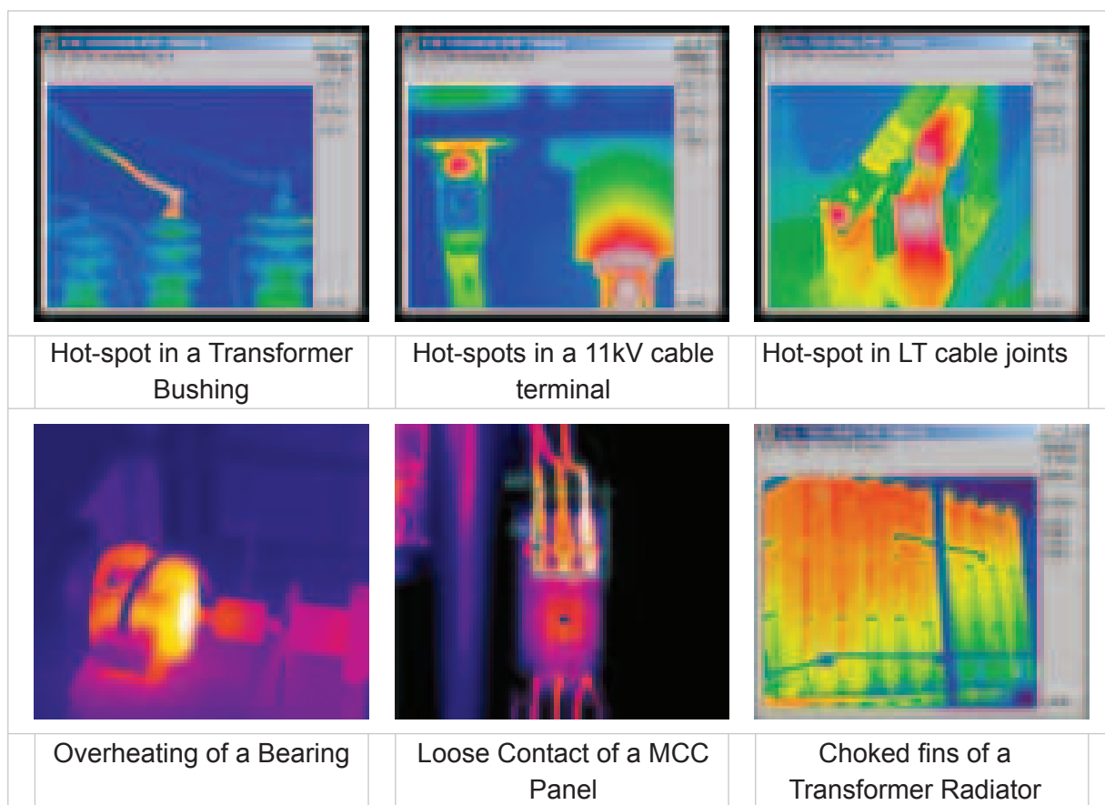
Figure 6.10 Thermographic measurement
