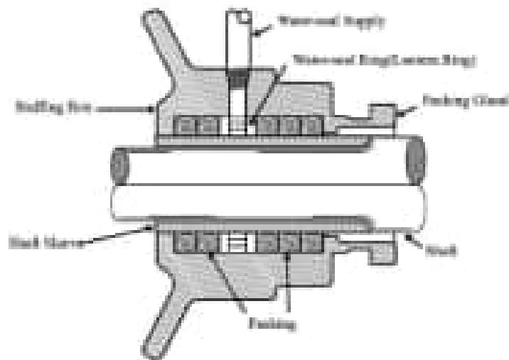
Figure 3.14 Packing gland
