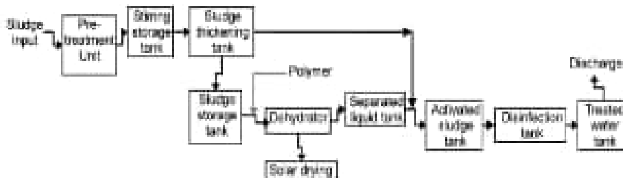
Figure 10.4 Flow chart of sludge treatment
