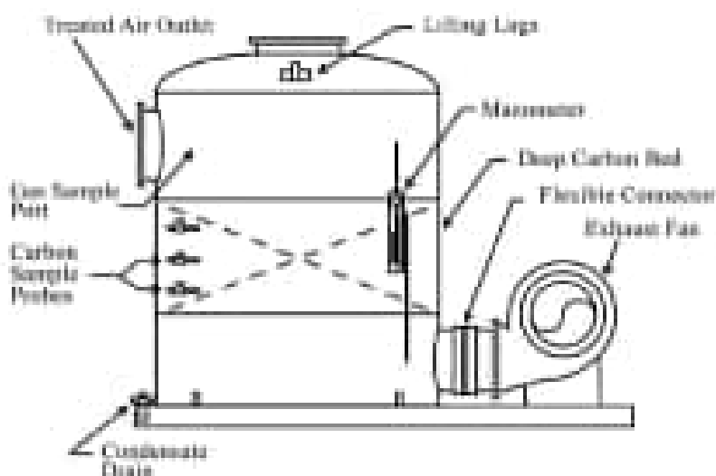
Figure 8.4 Activated-carbon deodorization
