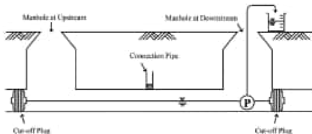
Figure 2.21 Pumping test
