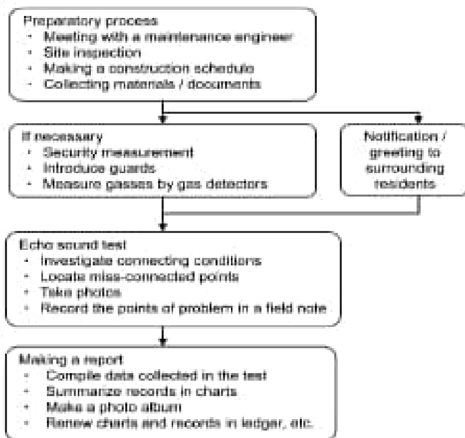
Figure 2.19 Work Procedure of Echo Sound Test
