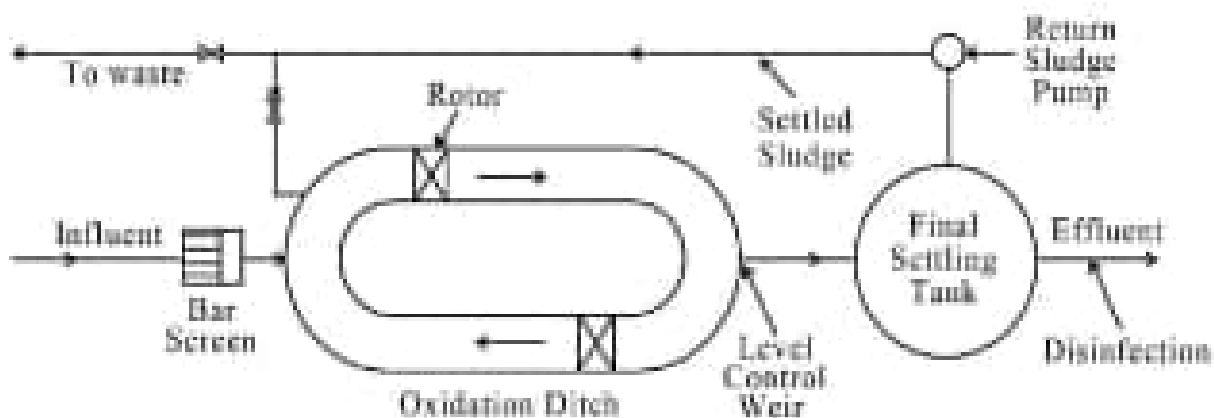
Figure 4.14 Oxidation ditch
