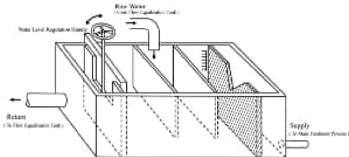
Figure 10.2 Metering unit
