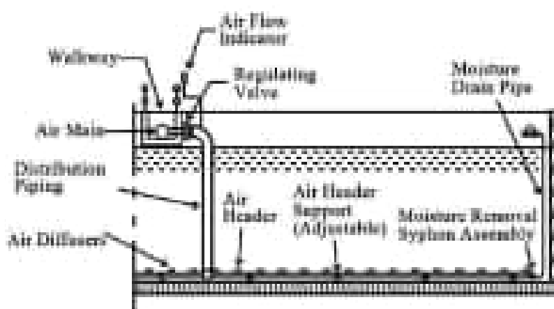
Figure 4.10 Typical air distribution system in aeration tank
