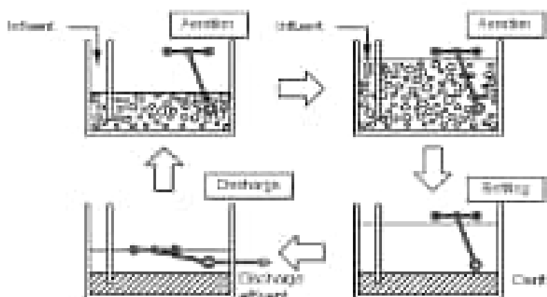
Figure 4.12 Operating cycles of intermittent SBR process
