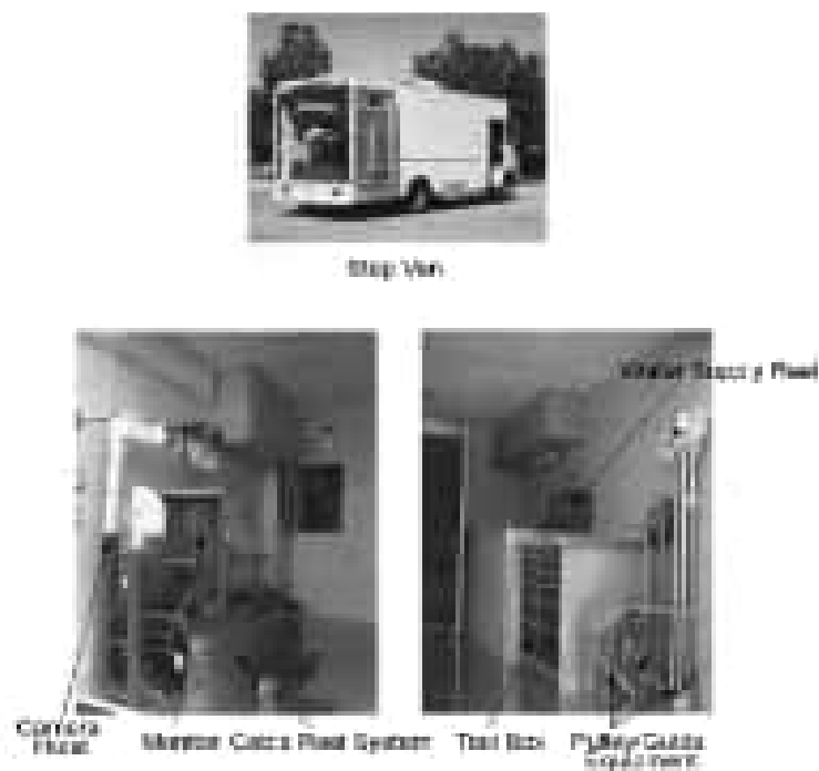
Figure 2.8 Step van CCTV system
