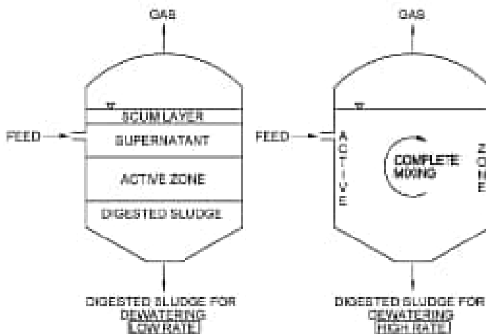
Figure 5.3 Sludge digestion system
