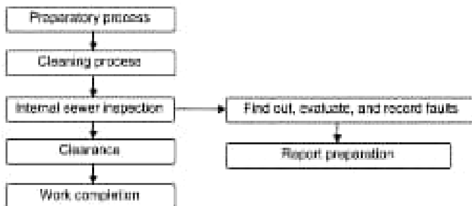
Figure 2.44 Work procedure for examination of lateral sewer by TV camera
