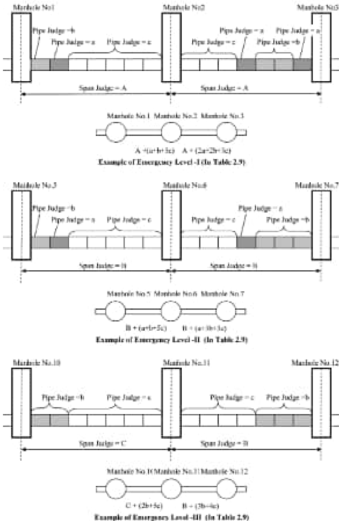
Figure 2.25 Illustration of testing criteria for sewer
