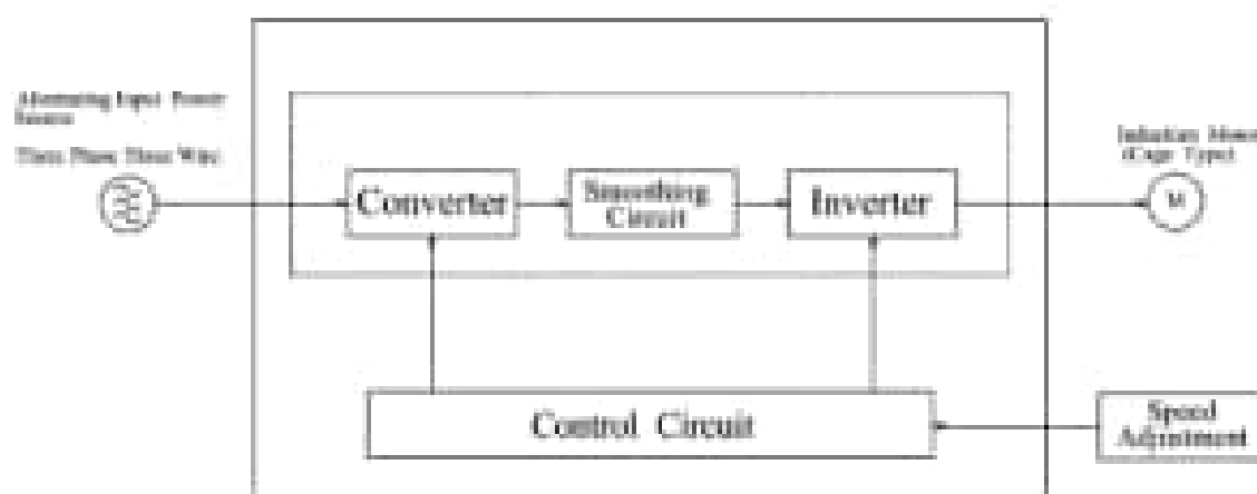
Figure 6.11 Variable Frequency Drive
