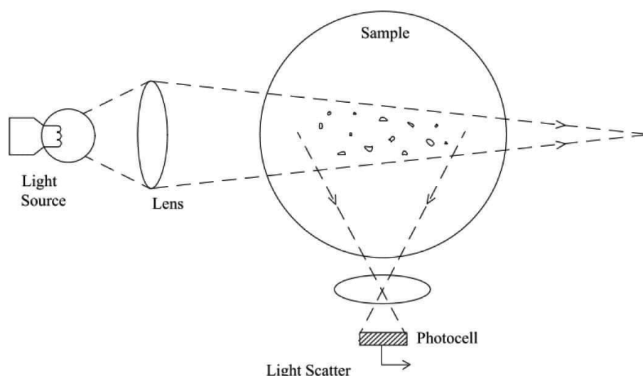
Figure 6.18 Nephelometer
