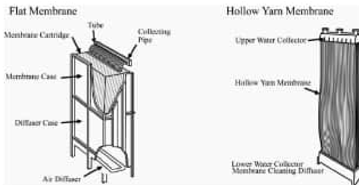
Figure 10.3 Membrane separators
