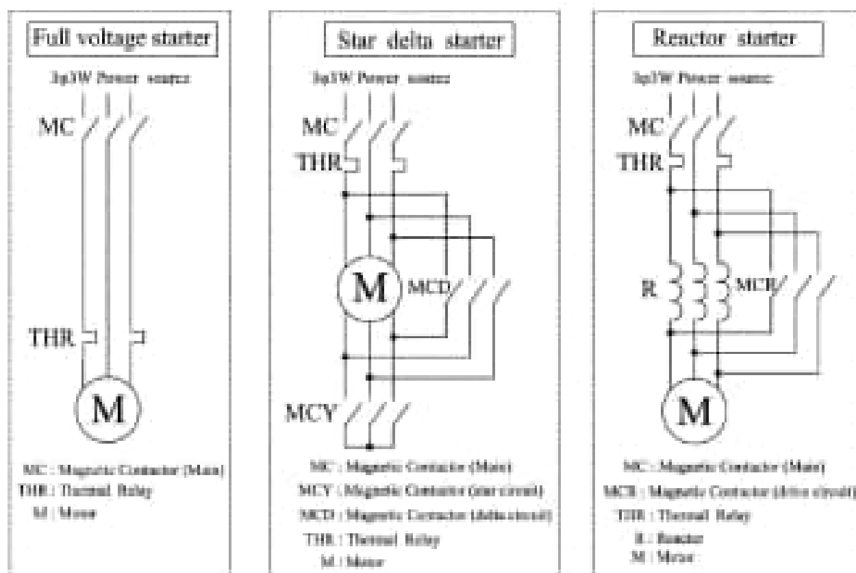
Figure 6.8 Starters
