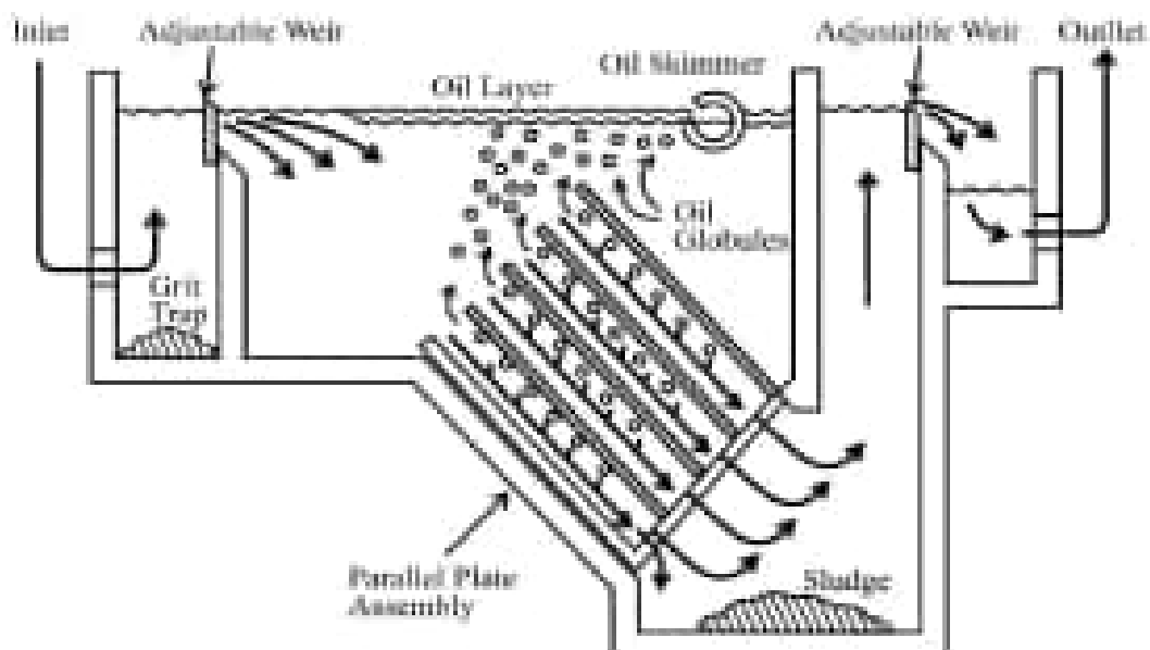
Figure 4.1 Typical gravity type oil and grease removal unit
