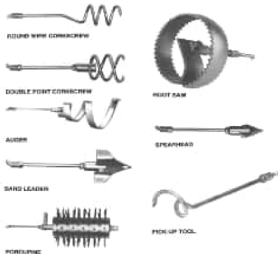
Figure 2.28 Rodding heads
