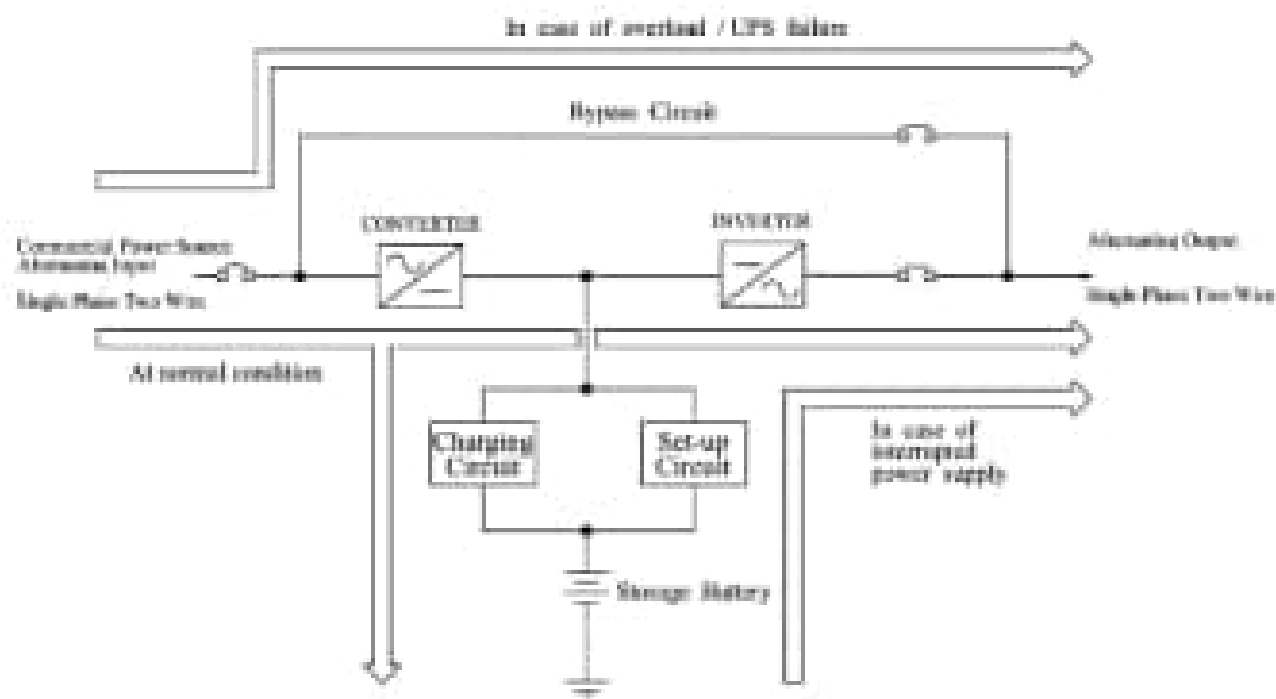
Figure 6.7 UPS circuit
