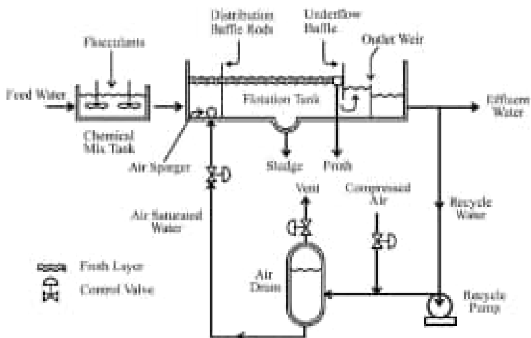
Figure 4.4 Schematic of DAF unit
