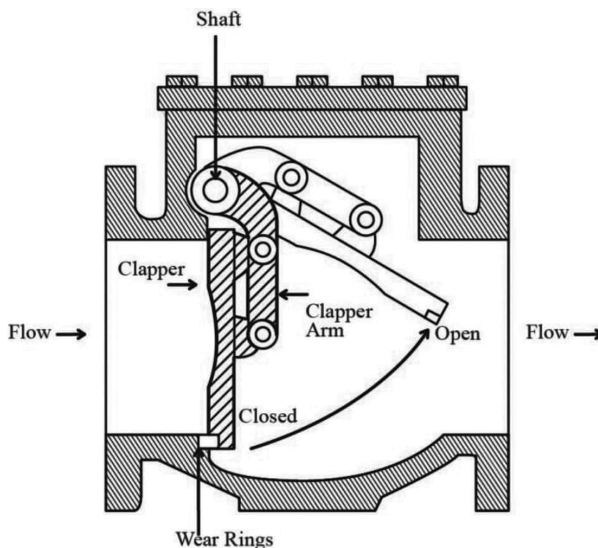
Figure 3.5 Check valve
