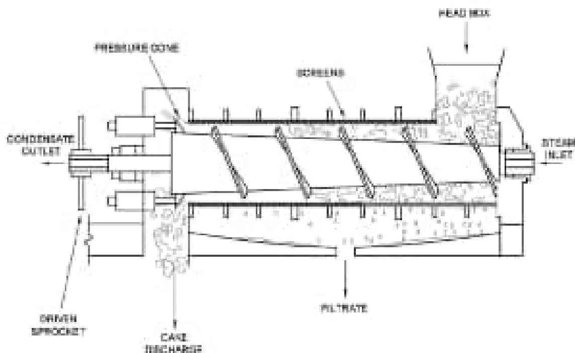
Figure 5.6 Screw press
